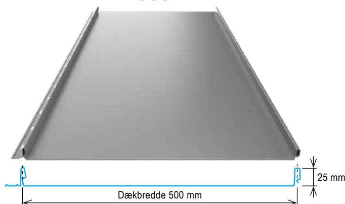
Easy-Clickfals 500
