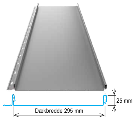
Easy-Clickfals 295
