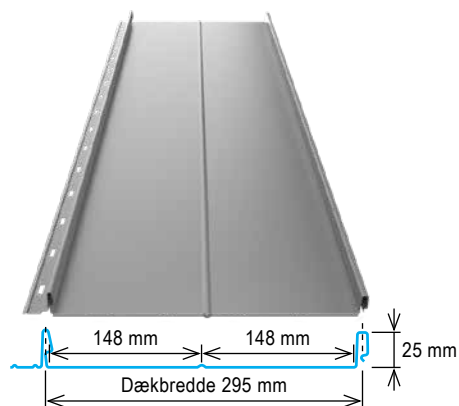
Easy-Clickfals 295-148
