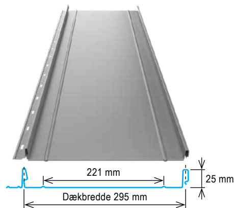
Easy-Clickfals 295-221
