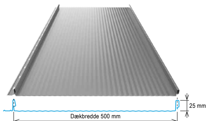
Easy-Clickfals 500-Micro
