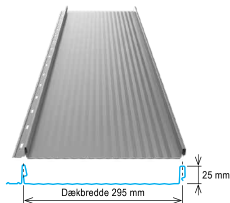
Easy-Clickfals 295-Micro
