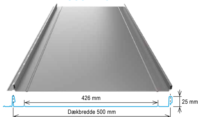
Easy-Clickfals 500-426
