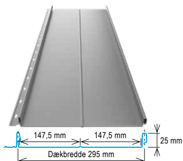
Easy-Clickfals 295-148
