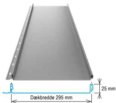
Easy-Clickfals 295-148
