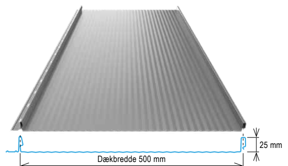
Easy-Clickfals 500-Micro
