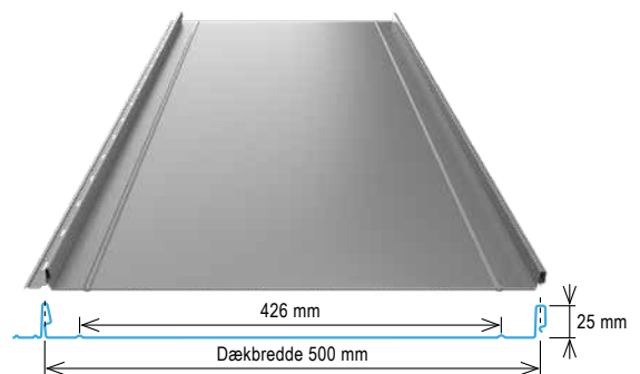
Easy-Clickfals 500-Micro
