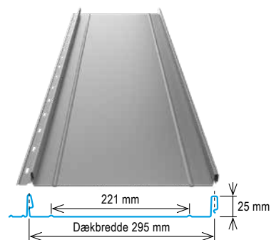
Easy-Clickfals 295-Micro
